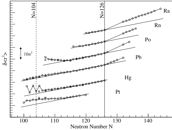
Fig. 6.4 Changes of the mean-square nuclear charge radii in the lead region. A constant offset was used for all isotopes of one element in order to separate the data points of the different elements, which would otherwise lay on top of each other. Thus, the \delta\langle r_c^2 \rangle axis is only to be taken relative. The straight lines represent the prediction from the spherical finite-range droplet model [42]. The kink at the N = 126 shell closure is clearly visible. Neutron-deficient isotopes of most elements exhibit also a deviation from this line due to deformation effects. Figure taken and modified from [44] including data from [45]
