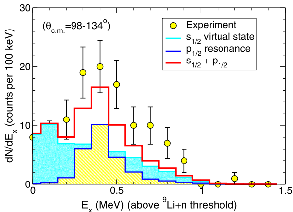
Fig. 2.4 Illustration of the transfer-to-the-continuum method, using a binning discretization, for the reaction {}^2\text{H}({}^9\text{Li}, p){}^{10}\text{Li}^*
