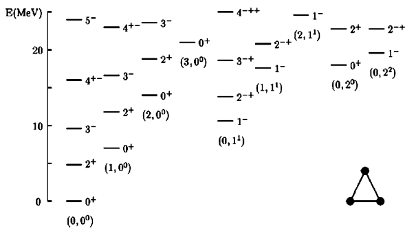
Fig. 1.15 Spectrum of the energy levels of an equilateral triangle configuration. The bands are labeled by (v_1; v_2^l) [66]
