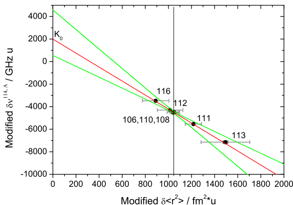
Fig. 6.2 Modified King plot for stable cadmium isotopes in the 5s\ ^2S_{1/2} \rightarrow 5p\ ^2P_{3/2} transition in \text{Cd}^+ . Small error bars reflect the statistical uncertainties whereas the large horizontal error bars are due to systematic uncertainties. A linear fit allows to determine the mass shift constant from the crossing with the y axis and the slope is determined by the field shift constant F . The 1\sigma confidence band is also shown
