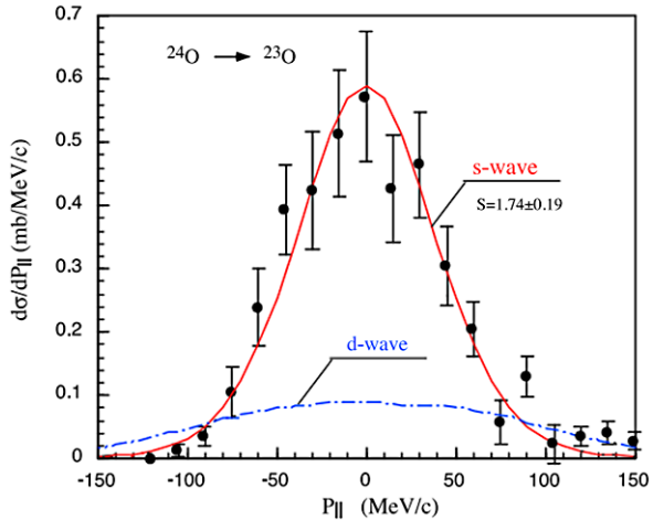
Fig. 5.16 Longitudinal momentum distribution after one-neutron removal from ^{24}\text{O} . The solid curves correspond to the eikonal model for neutron knockout from 2s_{1/2} in red, and 1d_{5/2} in blue [49]. Figure extracted from [49]
